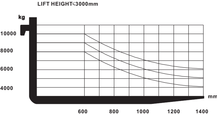
Load chart
