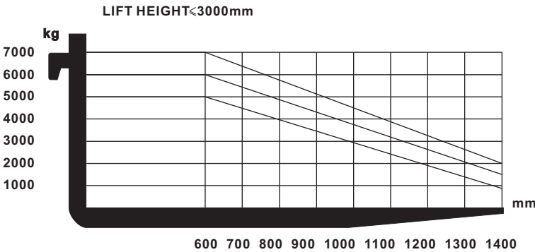
Load chart
