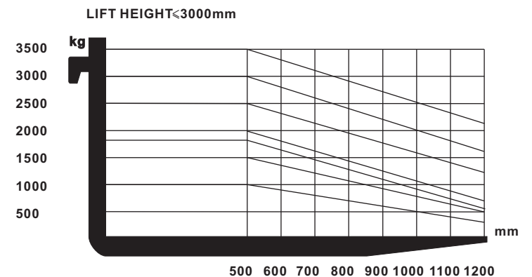
Load chart
