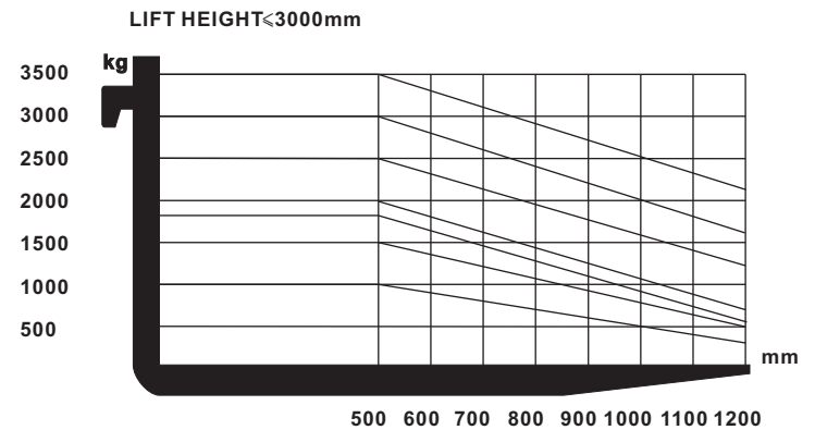
Load chart
