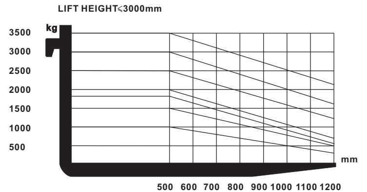
Load chart
