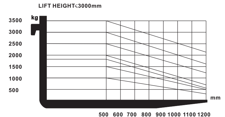
Load chart
