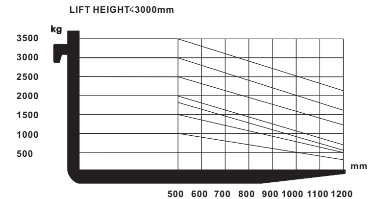
Load chart
