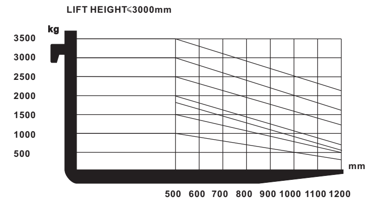
Load chart
