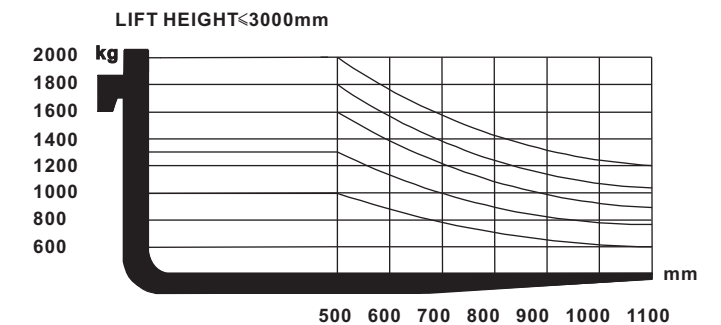
Load chart
